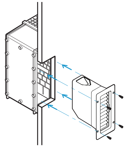
Screw fix the body into the wall.
