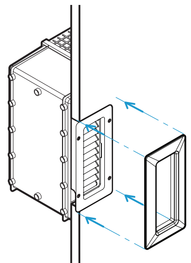
Snap fit the cover plate into position.
