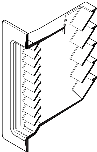
Showing the two layers of louvre.
